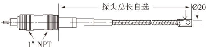
缆式探头L863CW
